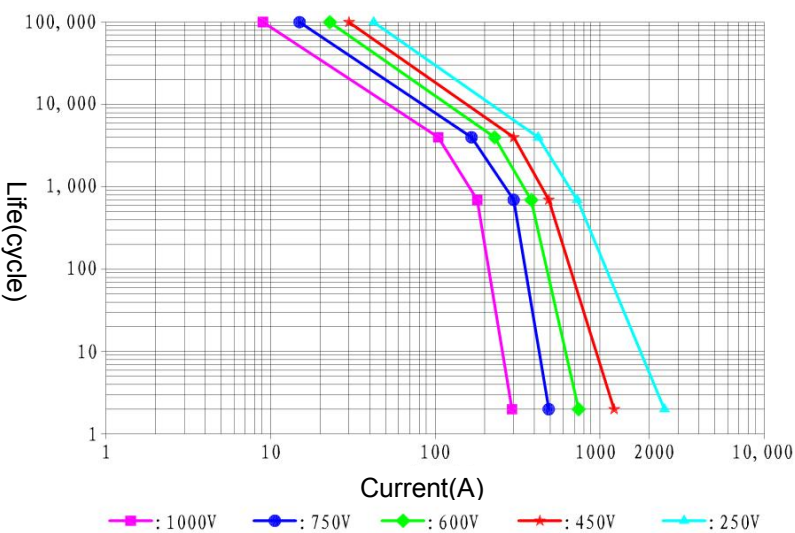
Cut-off life curve of resistive load
