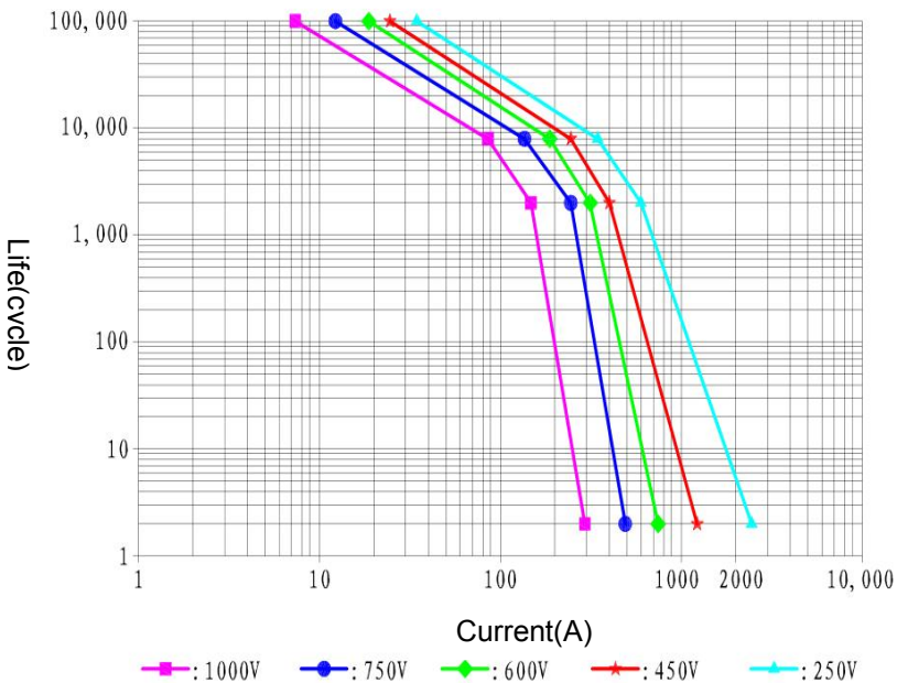
Cut-off life curve of resistive load
