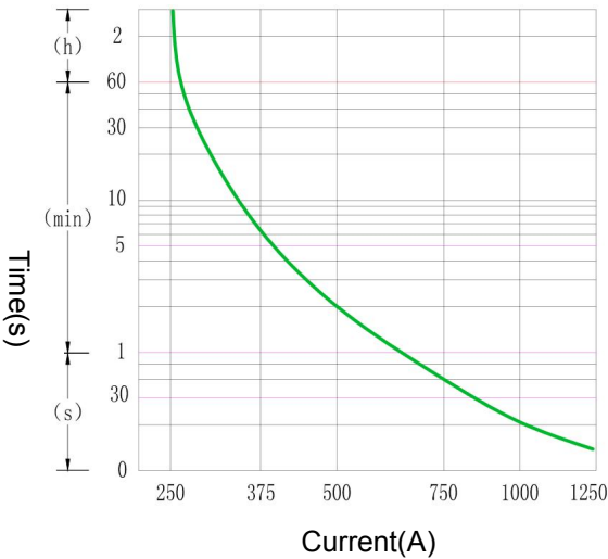
Short overload capacity curve
